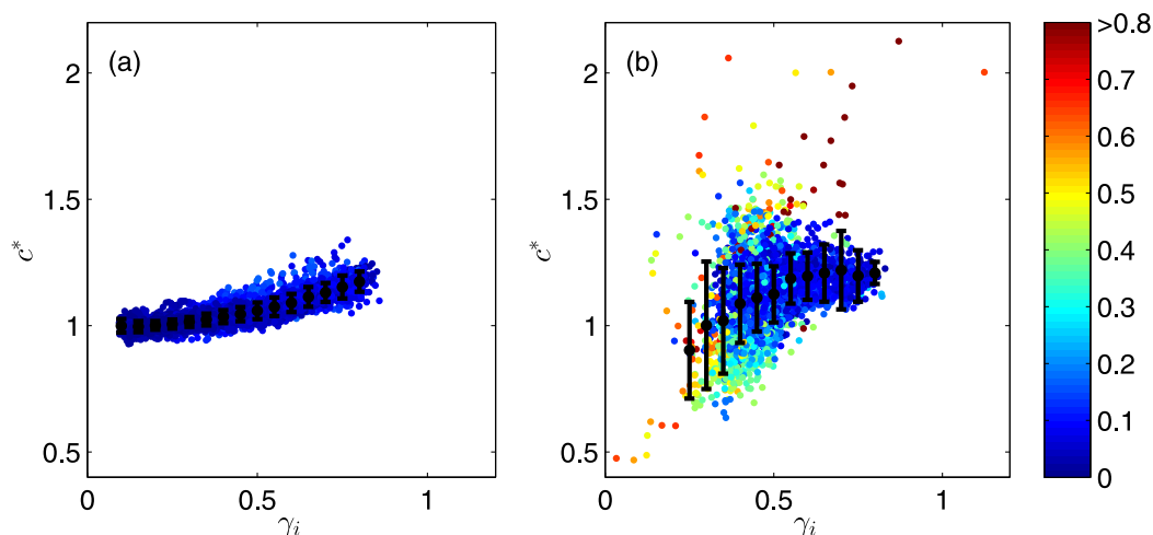
Figure 5. Normalized celerity c^* = c_i/c_{lin} as a function of the relative wave height \gamma_i = H_i/h_i for the 11 wave experiments. (a) Shoaling wave celerity only (6119 celerity estimates) and (b) breaking and broken waves only (3346 estimates). The data are divided into bins based on the value of \gamma_i ( \gamma_i between 0.05 and 1.5, with a step of 0.05). The black dots are mean c^* values for these data bins (only the bins where n \geq 10 are shown). The error bars are \pm 1 standard deviations per bins. The colors of the scatterplot indicate the value of the root-mean-square infragravity-wave height to water depth ratio H_{rms,lf}/\bar{h} at the location where the celerity were measured.
