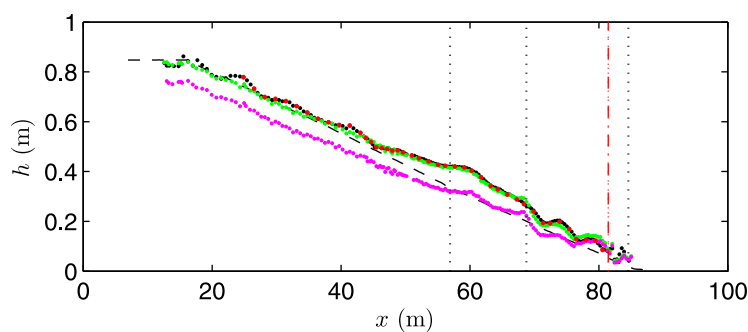
Figure 12. Depth estimates (dots) and measured water depth (dashed line) for case G3. Black dots: average of the individual water depths \bar{h}_i , where \bar{h}_i is calculated based on linear theory from c_i and T_i . Red dots: same calculation, but accounting for the infragravity-wave current, i.e., \bar{h}_i calculated from c_i - u_i . Green dots: depth calculated from c_{Xcor} and \bar{T} using linear theory. Magenta dots: depth estimated from c_{Xcor} , \bar{T} and \bar{H} using Booi's celerity predictor (equation (7)). The red dash-dotted line indicates the position where waves start merging. See caption of Figure 1 for definition of the vertical dotted lines.
